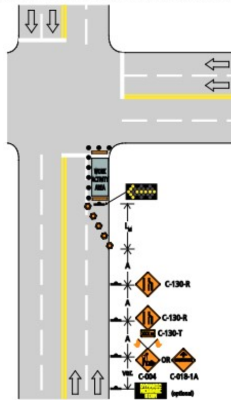
Figure 11.8: Right Lane Closure (Near Side) – Multilane Intersection – Short and Long Duration
